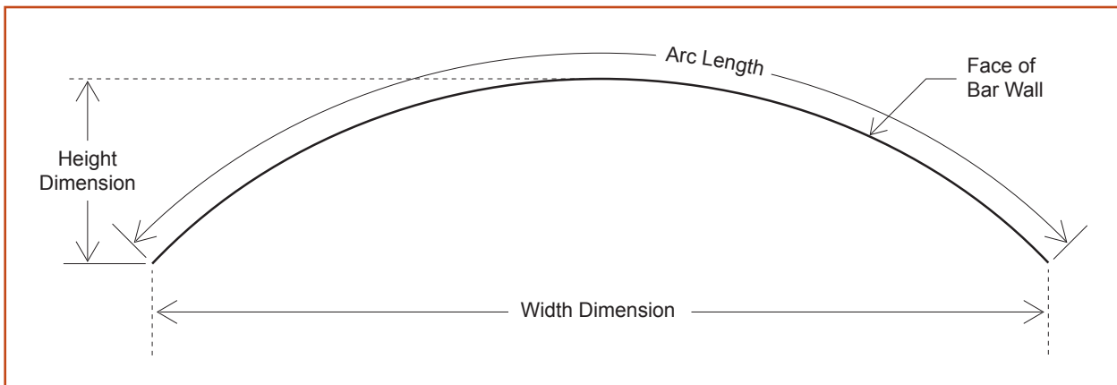
Figure 1. Use the diagram to measure the width, height, and arc length of larger sweeping curve.
