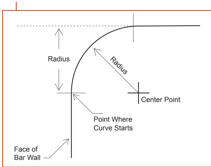
Figure 2. Use the diagram to measure the radius of a 90° corner.
